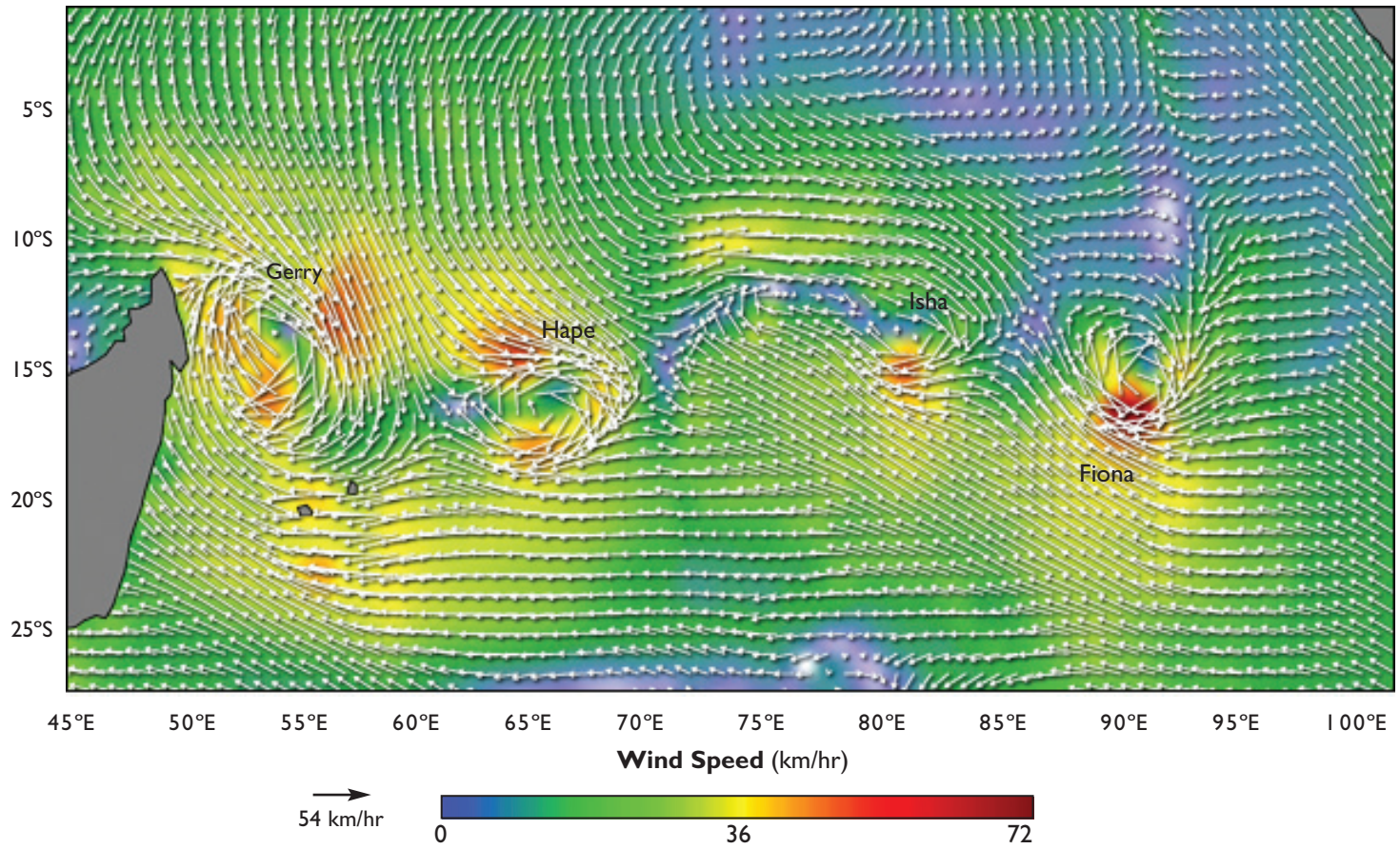
Wind direction and speed in the Indian Ocean, February 11, 2003. Wind direction (white arrows) is superimposed on a color map of wind speed. The figure demonstrates the details of 4 tropical cyclones revealed by 2 scatterometers flying in tandem. (Data from the SeaWinds instruments on the QuikScat and ADEOS II satellites.)
