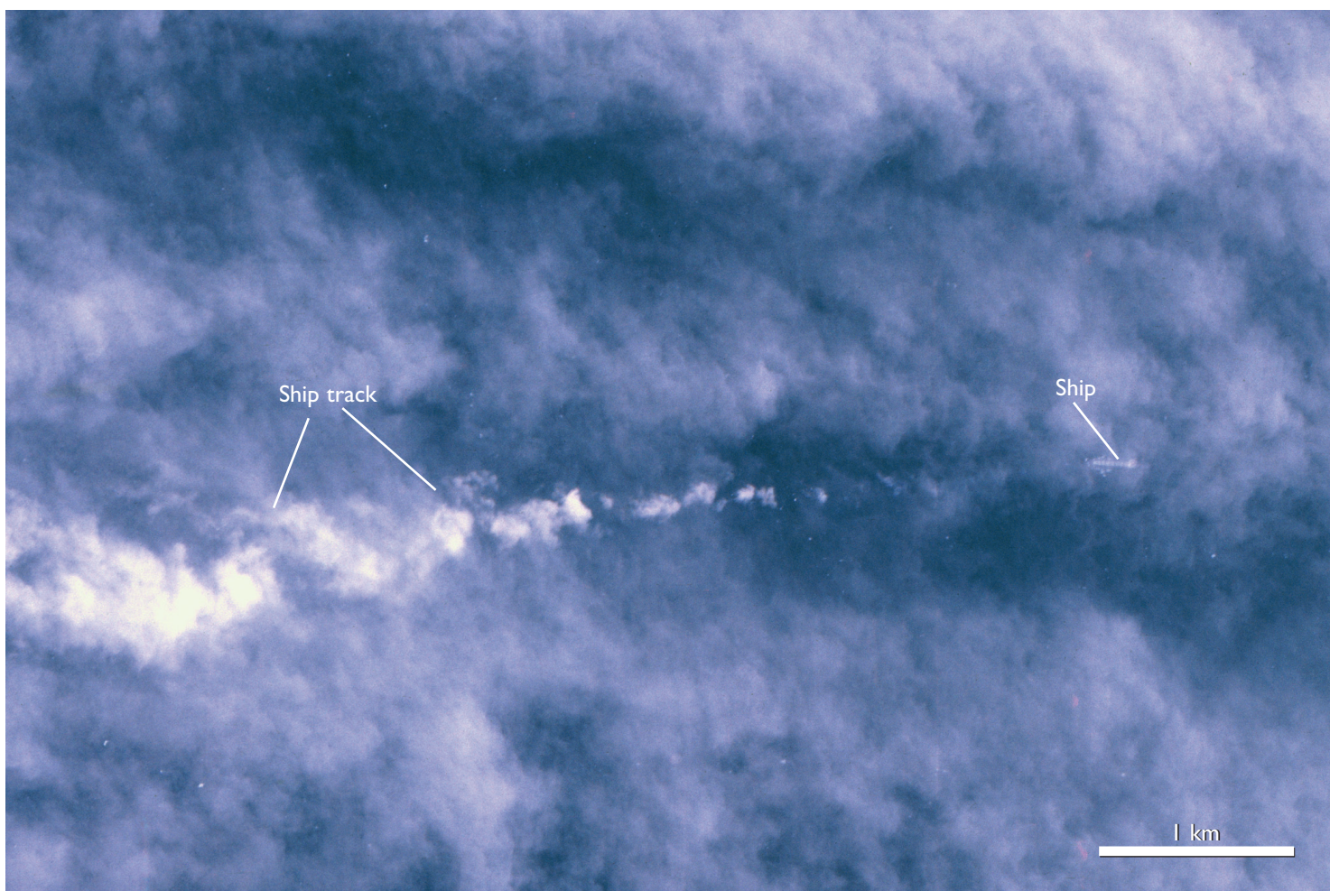
Photograph of a container ship off Monterey, California on June 13, 1994 and the resulting ship track produced downwind of the ship from condensation onto particles produced by the ship exhaust. An approximate length scale is shown. (Photograph from the RC-10 camera on NASA ER-2 aircraft.)
