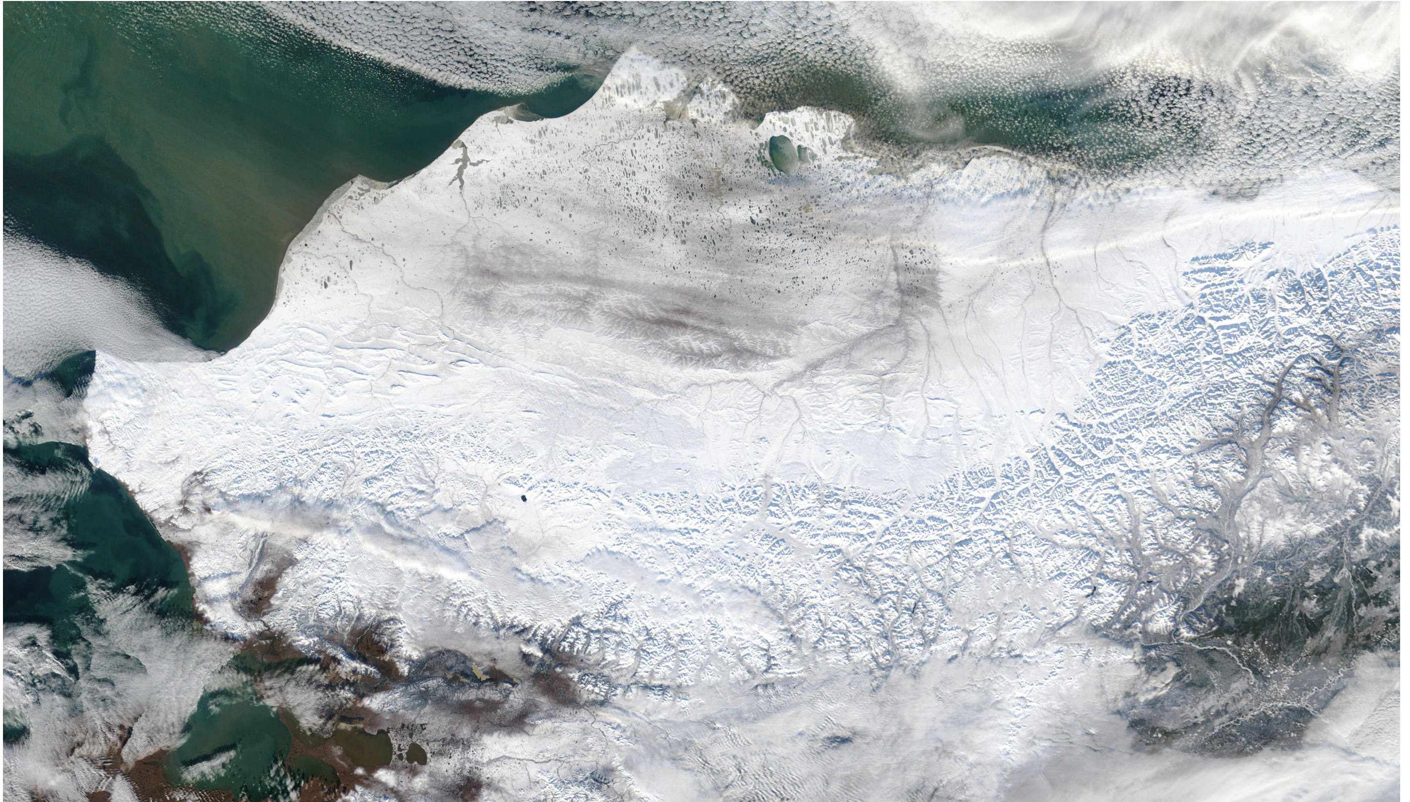
Snow cover and thaw lakes in northern Alaska, October 15, 2002. The Brooks Range is also visible on the image. (Data from the MODIS instrument on the Terra satellite; image courtesy of the MODIS Rapid Response Team, NASA Goddard Space Flight Center.)
