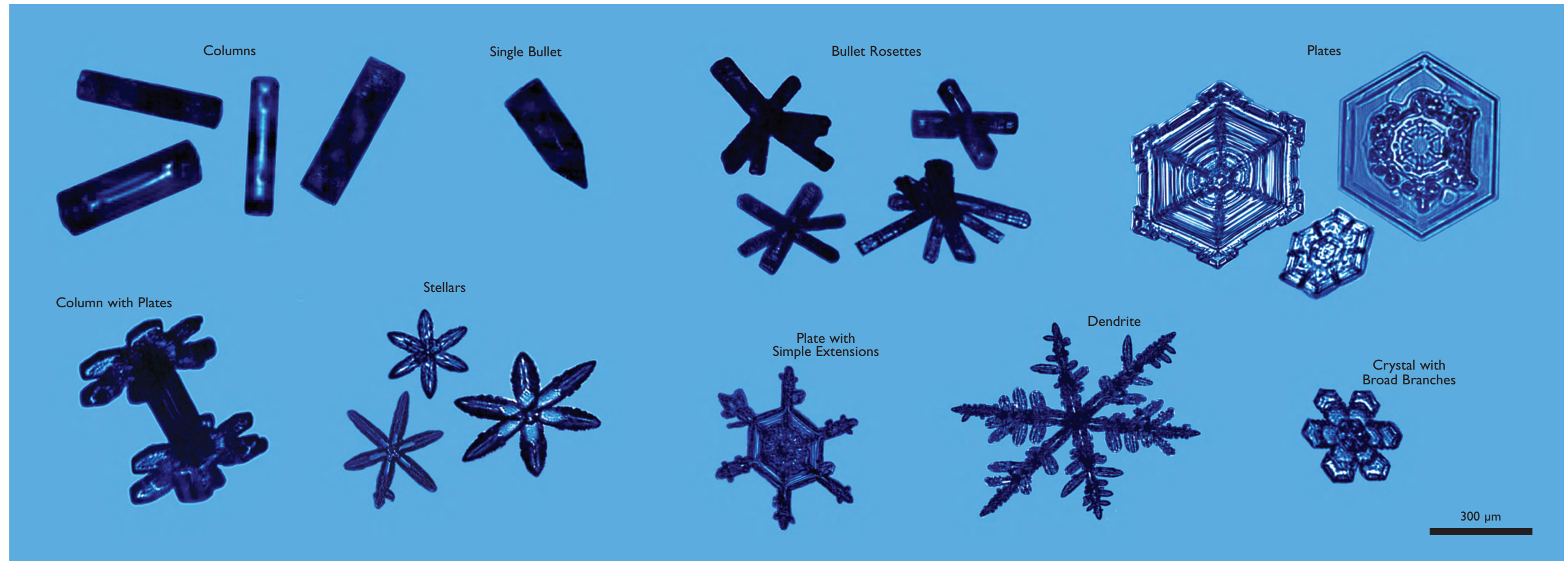
Digital images of ice crystals in clouds. A broad range of temperatures and humidities in clouds lead to the growth of different ice crystal shapes, which scatter light in widely different patterns. (Data from the CPI instrument on the SPEC Learjet, provided by Paul Lawson.)
