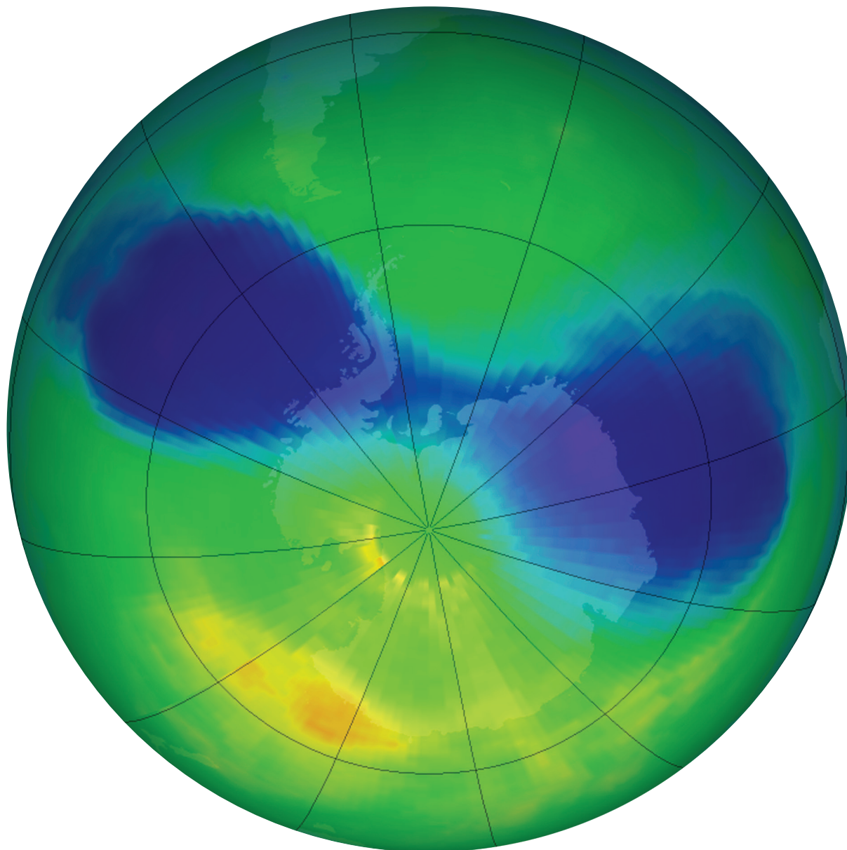
Total Ozone Content (Dobson Units)
