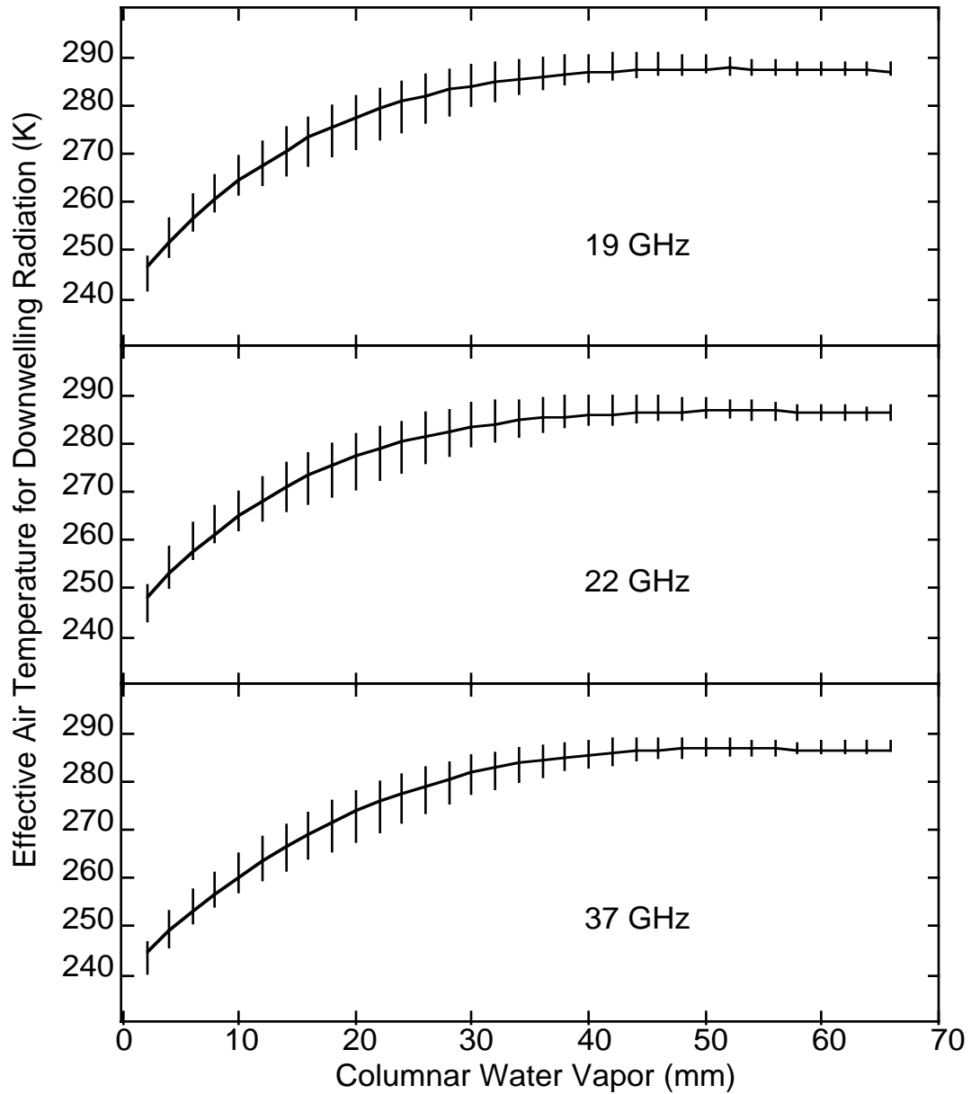
Fig. 4. The effective air temperature T_D for downwelling radiation plotted versus the RAOB columnar water vapor. The solid curve is the model value, and the vertical bars are the \pm one standard deviation of T_D derived from radiosondes.
