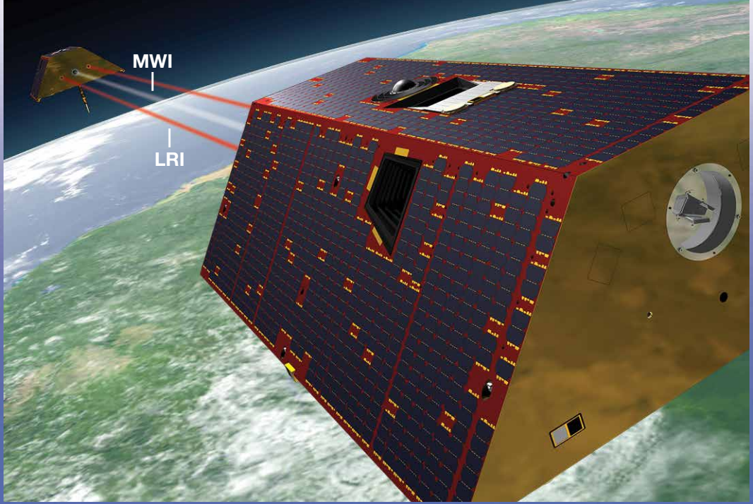
[Above] The experimental Laser Ranging Interferometer (LRI) is expected to provide better ranging precision than GRACE's MWI system. LRI is being tested on GRACE-FO as an enabling technology for the next-generation of mass change missions.
