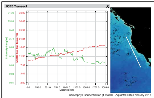
Comparison of sea surface temperature and chlorophyll concentrations.
